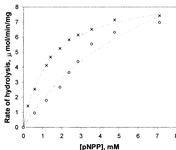
FIGURE 6: Presence of the fusion tag perturbs the kinetics of MDP-1 resulting in a higher K_M for p NPP. Assay conditions are described under Materials and Methods. N-glycyl-MDP-1 was prepared as indicated in the text. (x), N-glycyl-MDP-1; (o), CBP-MDP-1.
